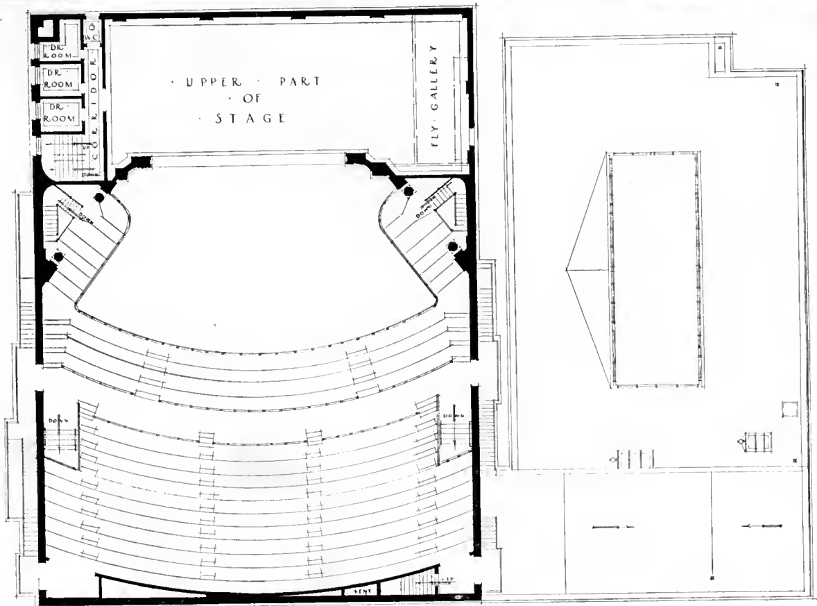
VIEW LOOKING ACROSS BALCONY AND BALCONY FLOOR PLAN BROADWAY THEATRE, SOUTH BOSTON, MASS. BLACKALL, CLAPP & WHITTEMORE, ARCHITECTS
